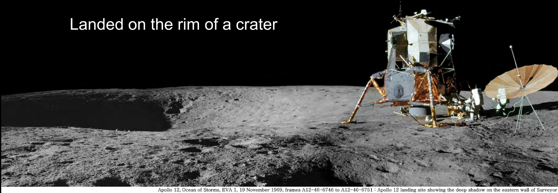
Apollo 12, Ocean of Storms, EVA 1, 19 November 1969, frames A12-46-6746 to A12-46-6751 : Apollo 12 landing site showing the deep shadow on the eastern wall of Surveyor Crater
